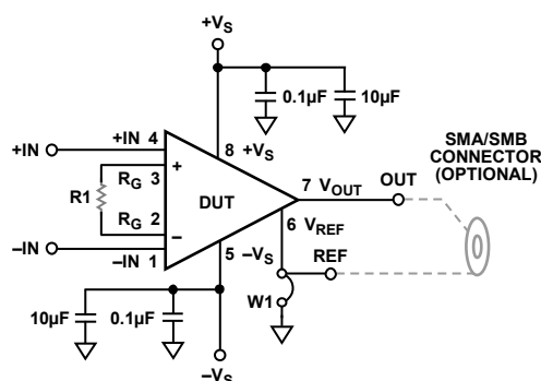
Figure 4. EVAL-INAMP-82RZ Schematic
