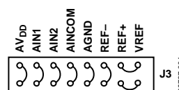
Figure 4. Connecting an Absolute Reference to the AD7195
