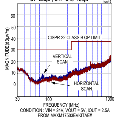
RADIATED EMISSION PLOT C4=C14=OPEN, L1=SHORT C7=220pF, C17=C18=150pF
