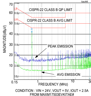
CONDUCTED EMISSION PLOT WITH FILTER: C4=2.2μF, L1=10μH, C14=2.2μF
