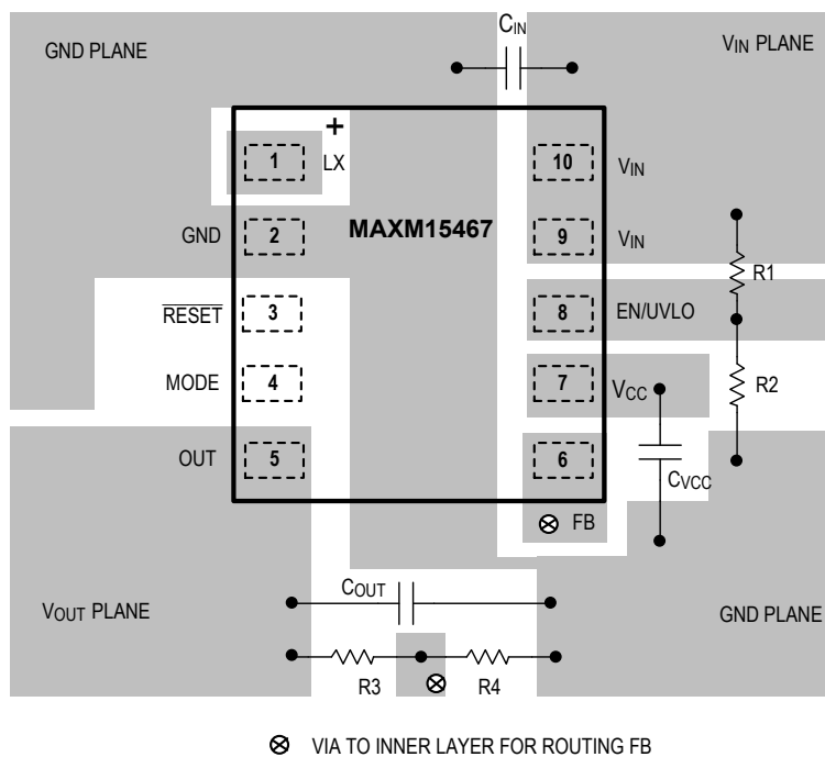
Figure 3. Adjustable Output Layout Guidelines
