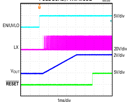
MAXM15467 STARTUP THROUGH ENABLE V_{IN} = 24V , ADJUSTABLE V_{OUT} = 3.3V , FULL LOAD, PWM MODE
