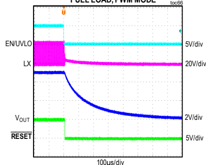
MAXM15466 SHUTDOWN THROUGH ENABLE
