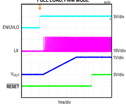
MAXM15467 STARTUP THROUGH ENABLE V_{IN} = 12V , ADJUSTABLE V_{OUT} = 1.5V , FULL LOAD, PWM MODE
