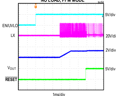
MAXM15465 STARTUP THROUGH ENABLE (2V PREBIAS)
