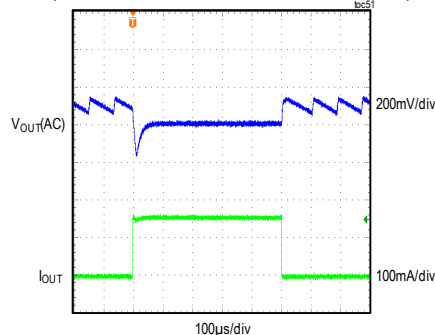
MAXM15466 LOAD TRANSIENT RESPONSE V_{IN} = 24V , FIXED V_{OUT} = 5V , PFM MODE (LOAD CURRENT STEPPED FROM 5mA TO 150mA)
