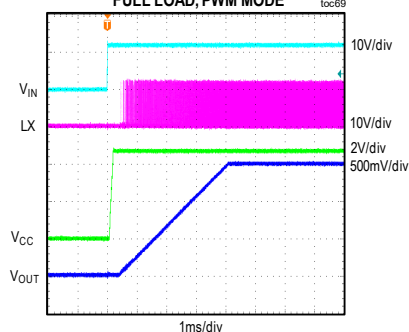
MAXM15467 STARTUP THROUGH V_{IN}
