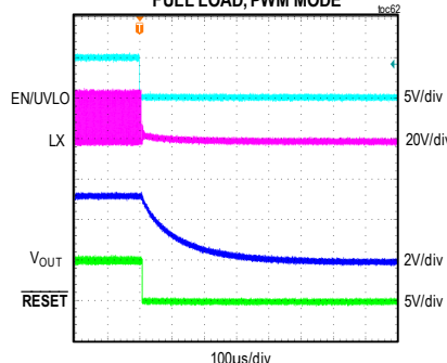
MAXM15465 SHUTDOWN THROUGH ENABLE V_{IN} = 24V , FIXED V_{OUT} = 3.3V , FULL LOAD, PWM MODE
