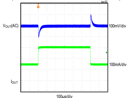
MAXM15466 LOAD TRANSIENT RESPONSE V_{IN} = 24V , FIXED V_{OUT} = 5V , PWM MODE (LOAD CURRENT STEPPED FROM 150mA TO 300mA)
