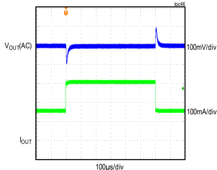
MAXM15467 LOAD TRANSIENT RESPONSE V_{IN} = 24V , ADJUSTABLE V_{OUT} = 3.3V , PWM MODE (LOAD CURRENT STEPPED FROM 150mA TO 300mA)
