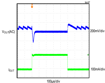
MAXM15467 LOAD TRANSIENT RESPONSE V_{IN} = 24V , ADJUSTABLE V_{OUT} = 5V , PFM MODE (LOAD CURRENT STEPPED FROM 5mA TO 150mA)
