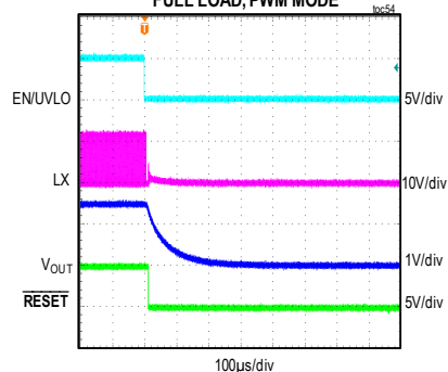
MAXM15467 SHUTDOWN THROUGH ENABLE V_{IN} = 12V , ADJUSTABLE V_{OUT} = 1.5V , FULL LOAD, PWM MODE
