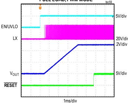
MAXM15467 STARTUP THROUGH ENABLE V_{IN} = 24V , ADJUSTABLE V_{OUT} = 5V , FULL LOAD, PWM MODE
