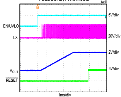
MAXM15465 STARTUP THROUGH ENABLE V_{IN} = 24V , FIXED V_{OUT} = 3.3V , FULL LOAD, PWM MODE
