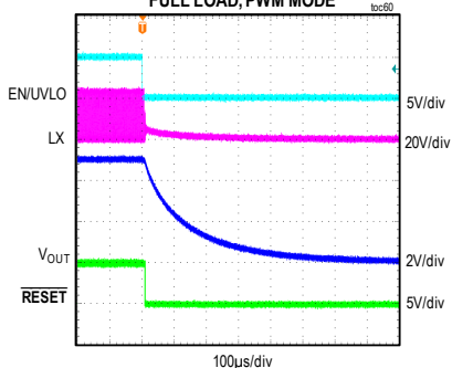
MAXM15467 SHUTDOWN THROUGH ENABLE V_{IN} = 24V , ADJUSTABLE V_{OUT} = 5V , FULL LOAD, PWM MODE
