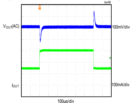
MAXM15467 LOAD TRANSIENT RESPONSE V_{IN} = 24V , ADJUSTABLE V_{OUT} = 5V , PWM MODE (LOAD CURRENT STEPPED FROM 150mA TO 300mA)
