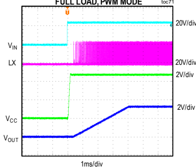
MAXM15467 STARTUP THROUGH V_{IN}
