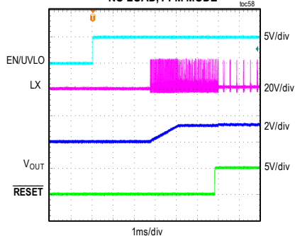
MAXM15467 STARTUP THROUGH ENABLE (2V PREBIAS) V_{IN} = 24V , ADJUSTABLE V_{OUT} = 3.3V , NO LOAD, PFM MODE
