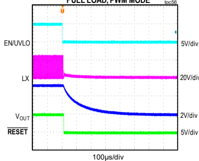
MAXM15467 SHUTDOWN THROUGH ENABLE V_{IN} = 24V , ADJUSTABLE V_{OUT} = 3.3V , FULL LOAD, PWM MODE
