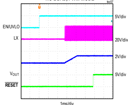
MAXM15467 STARTUP THROUGH ENABLE (2V PREBIAS) V_{IN} = 24V , ADJUSTABLE V_{OUT} = 3.3V , NO LOAD, PWM MODE
