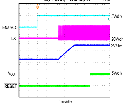
MAXM15466 STARTUP THROUGH ENABLE (2.5V PREBIAS)
