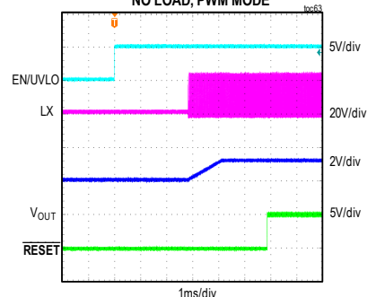
MAXM15465 STARTUP THROUGH ENABLE (2V PREBIAS) V_{IN} = 24V , FIXED V_{OUT} = 3.3V , NO LOAD, PWM MODE
