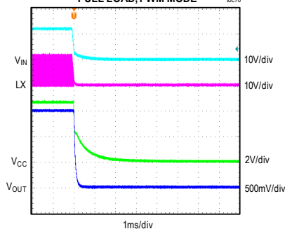
MAXM15467 SHUTDOWN THROUGH V_{IN}
