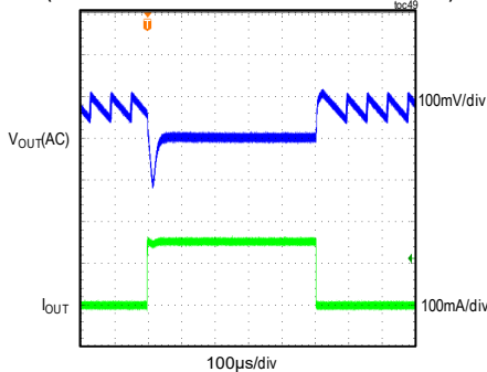
MAXM15465 LOAD TRANSIENT RESPONSE V_{IN} = 24V , FIXED V_{OUT} = 3.3V , PFM MODE (LOAD CURRENT STEPPED FROM 5mA TO 150mA)
