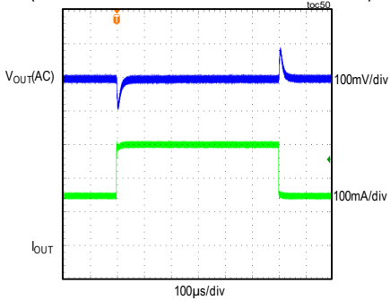
MAXM15465 LOAD TRANSIENT RESPONSE V_{IN} = 24V , FIXED V_{OUT} = 3.3V , PWM MODE (LOAD CURRENT STEPPED FROM 150mA TO 300mA)
