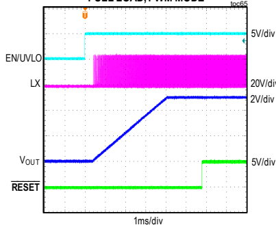
MAXM15466 STARTUP THROUGH ENABLE
