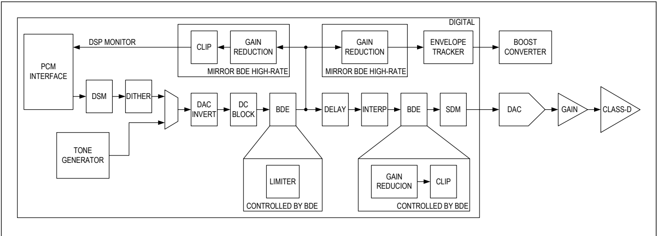
Figure 18. Amplifier Path
