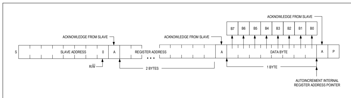
Figure 24. I 2 C Writing One Byte of Data to the Slave
