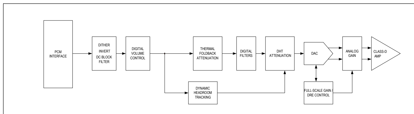
Figure 8. Speaker Amplifier Path
