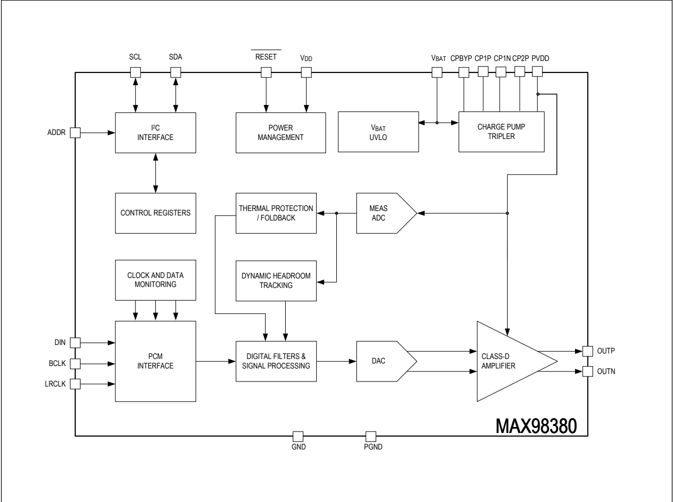
Detailed Block Diagram
