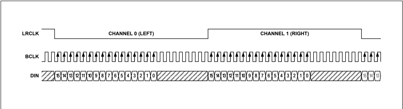
Figure 2. Left-Justified Mode
