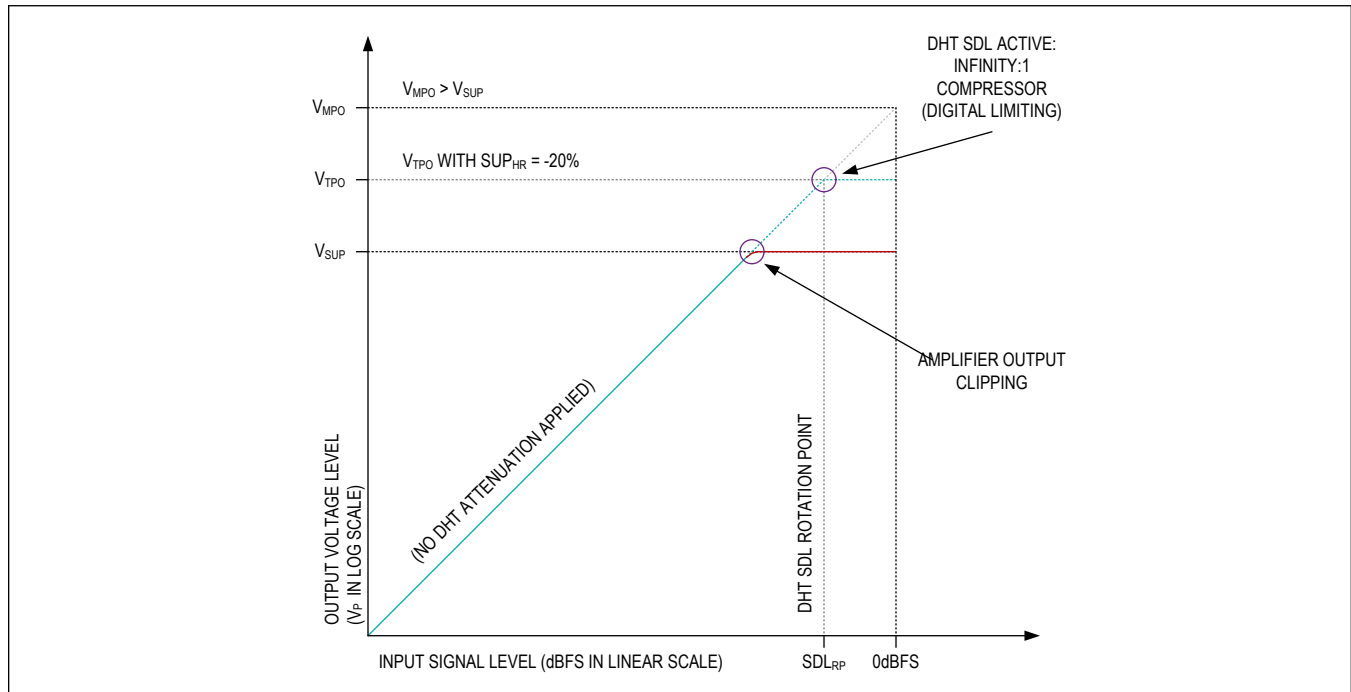
Figure 16. Signal Distortion Limiter with V_{\text{MPO}} > V_{\text{SUP}} and -20% Headroom ( \text{SUP}_{\text{HR}} )
