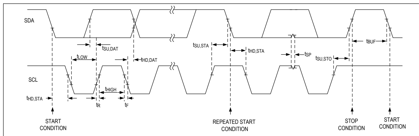
Figure 22. I 2 C START, STOP, and REPEATED START Conditions
