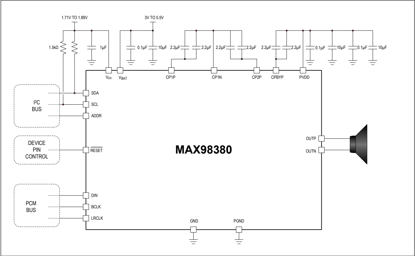
Typical Applications Circuit
