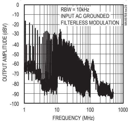
WIDEBAND OUTPUT SPECTRUM (FIXED-FREQUENCY MODULATION)
