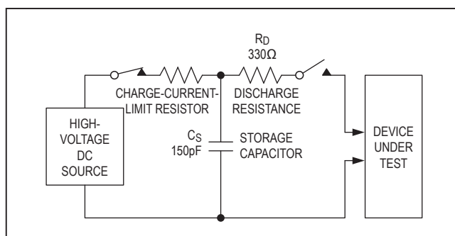
Figure 22. IEC 61000-4-2 Contact Discharge ESD Test Circuit
