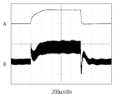
LINE-TRANSIENT RESPONSE
