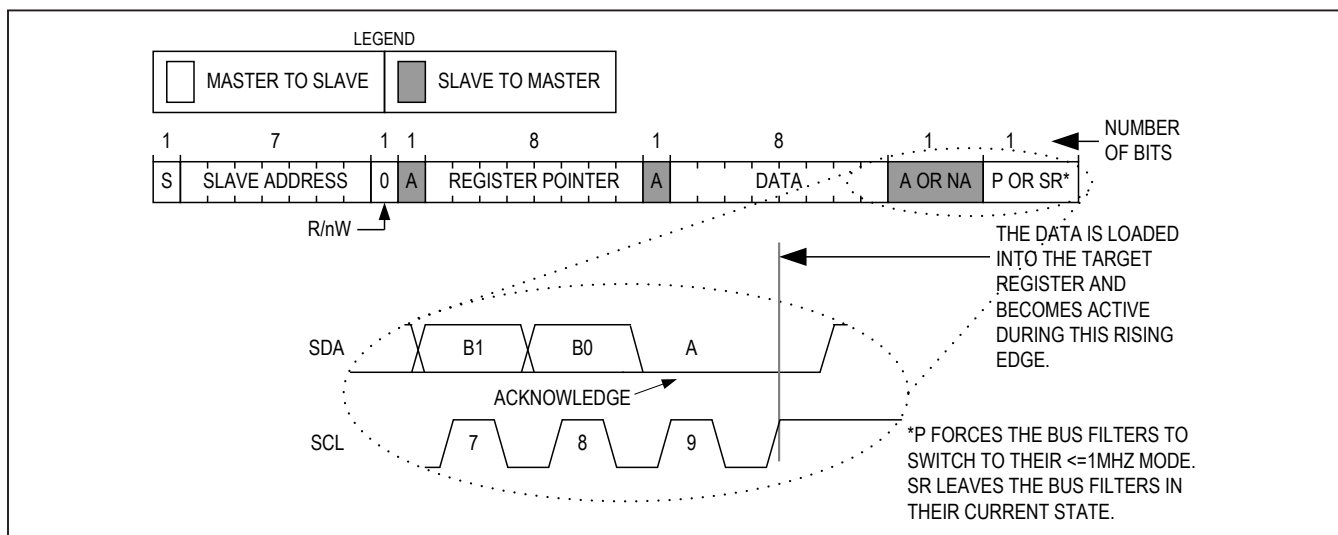
Figure 7. Writing to a Single Register with the Write Byte Protocol
