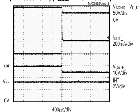
OVERCURRENT RESPONSE WAVEFORM (MAX5965AUAX) ( R_{LOAD} = 240\Omega TO 57\Omega )
