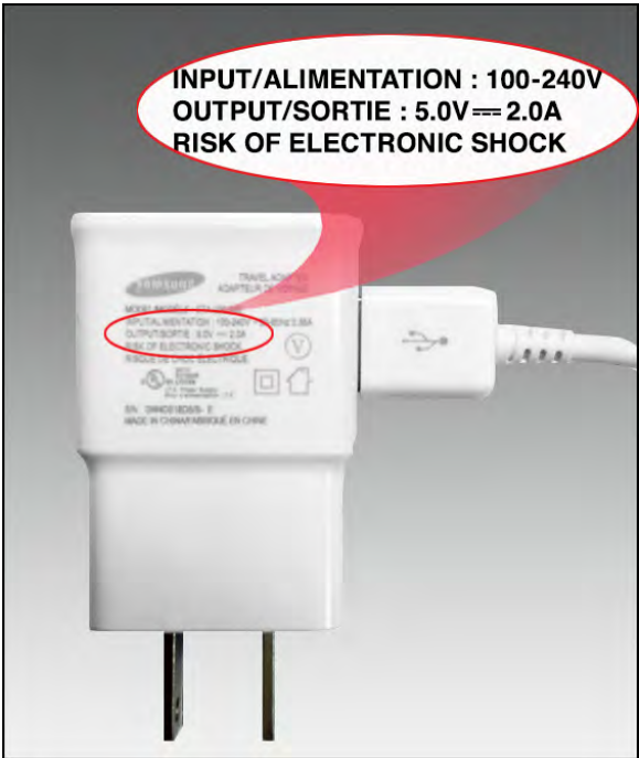
Figure 12. For More Power Delivered by USB Port Use a Wall Charger
