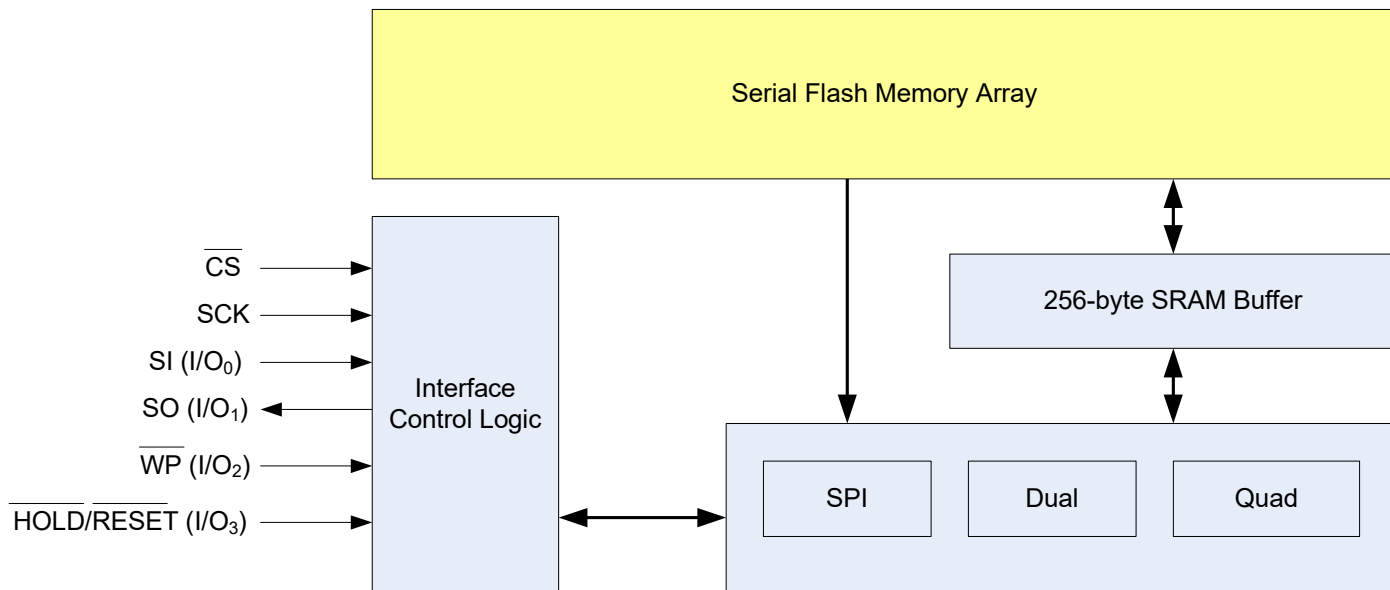
Figure 3-1. Block Diagram
