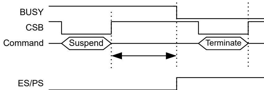
Figure 5-19. Allowing Enough Time for the Suspend Operation to Complete
