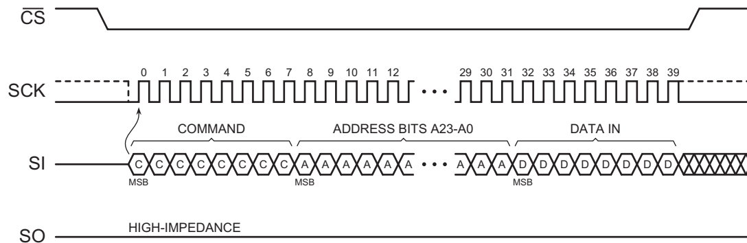
Figure 5-7. SPI Transfer — Command, Address, and Data — Write Operation
