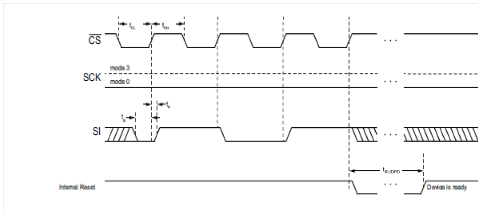
Figure 5-21. JEDEC Standard Hardware Reset
