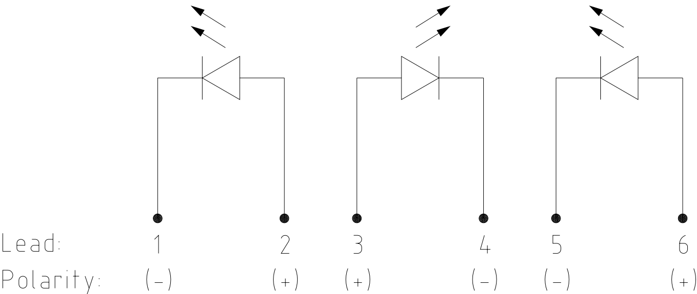
Circuit diagram
