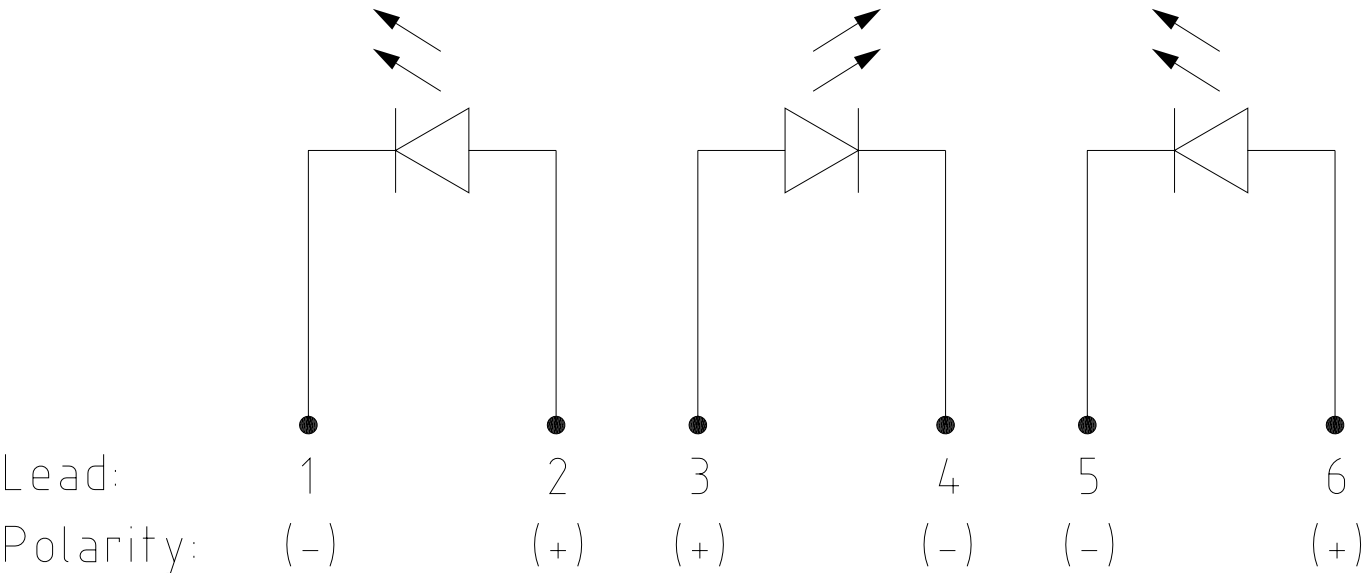
Circuit diagram
