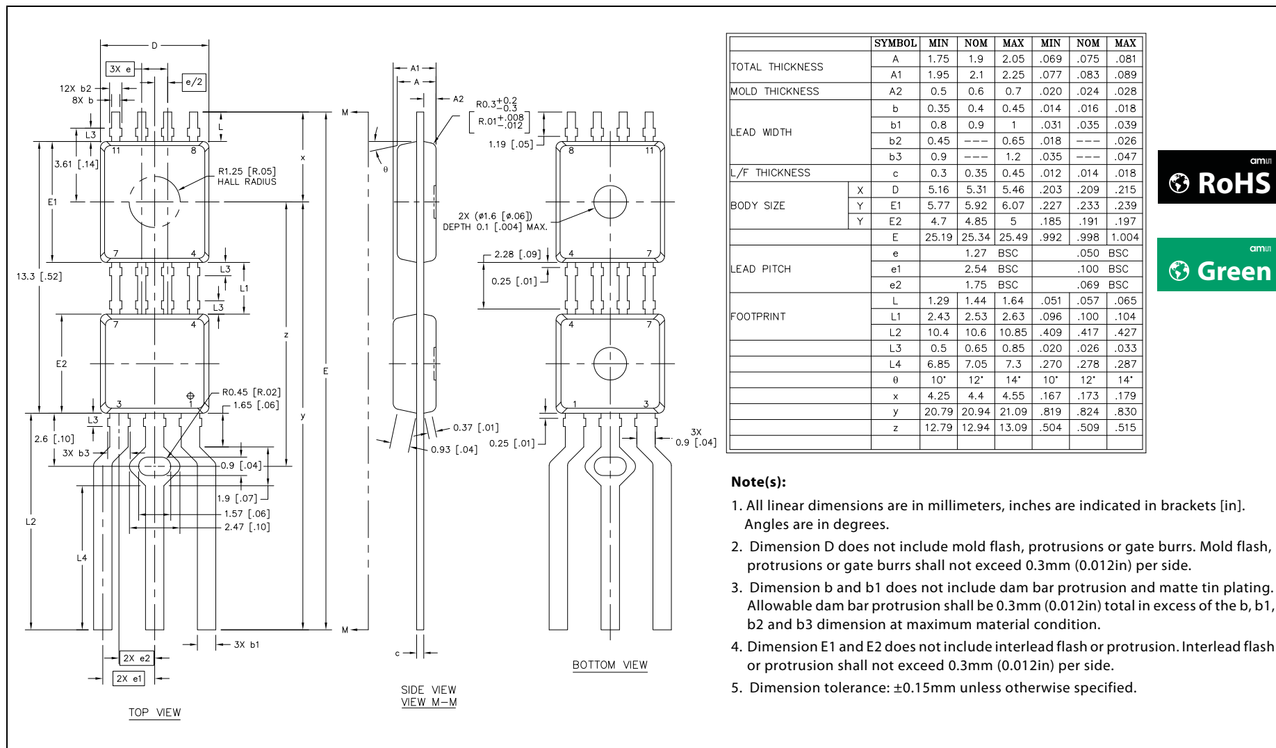
Figure 75: SIP Packaging Outline Drawing
