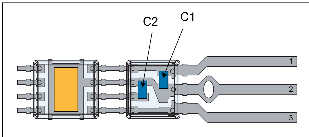
Figure 73: AS5172E/F Components
