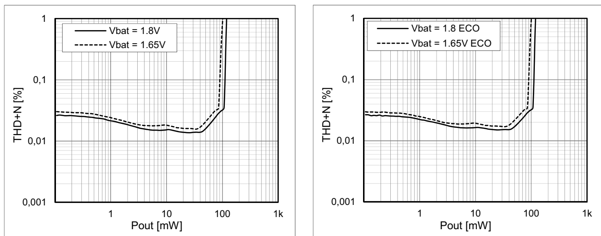
Figure 26: Headphone THD+N vs. Output Power 32 \Omega Mono
