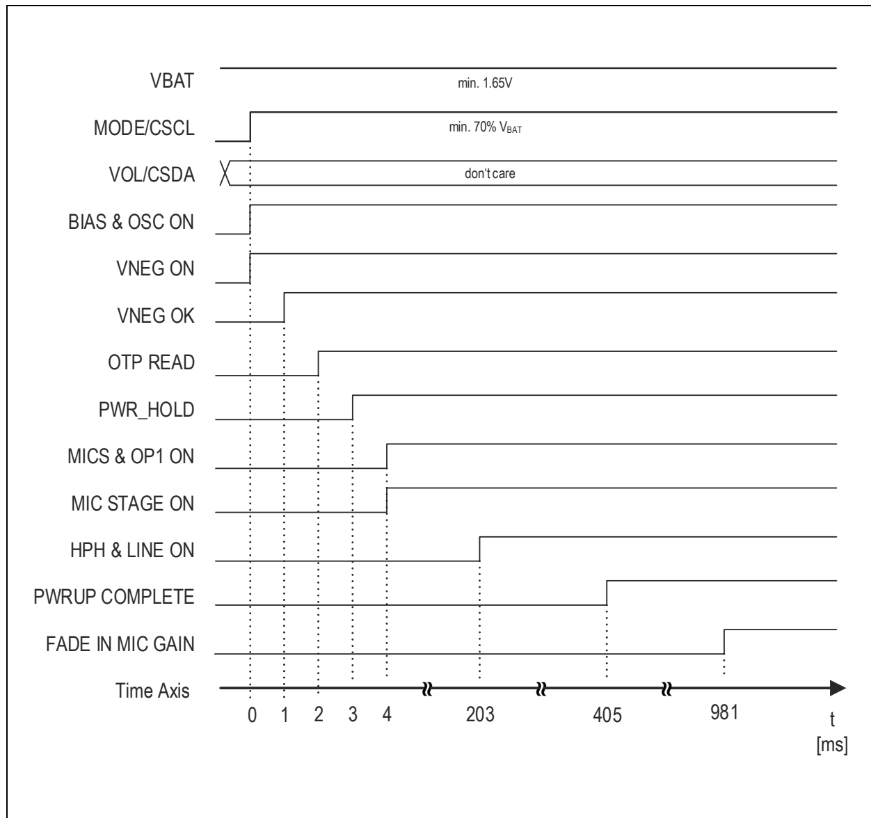
Figure 40: Start-Up Sequence
