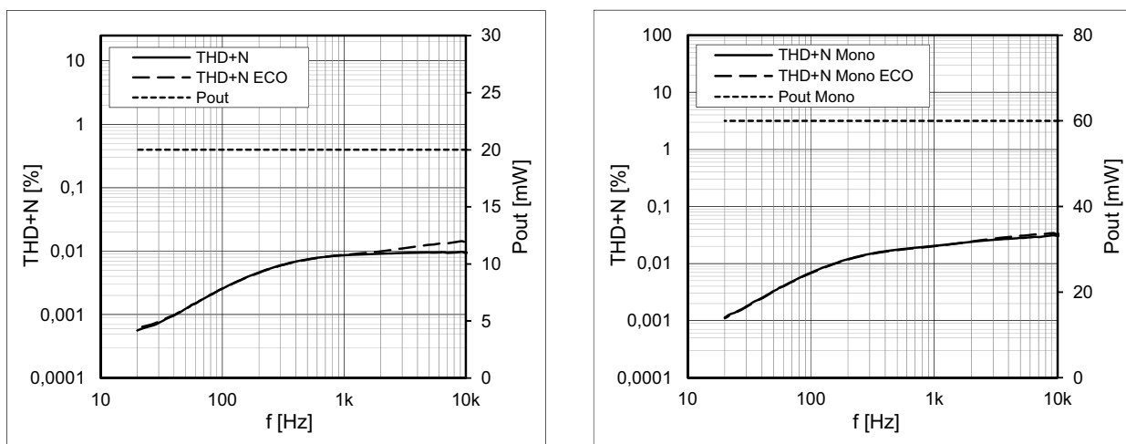
Figure 27: Headphone THD+N vs. Frequency 32 \Omega Stereo/Mono
