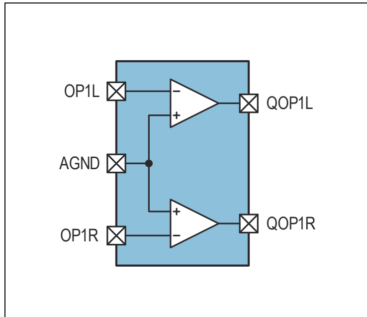
Figure 34: Operational Amplifiers
