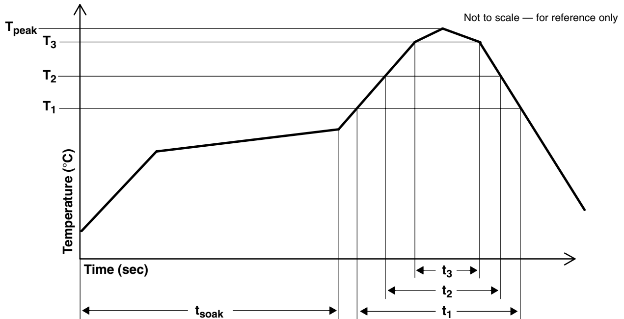
Figure 31. TSL2562/TSL2563 Solder Reflow Profile Graph
