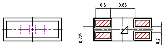
Component Location on Pad
