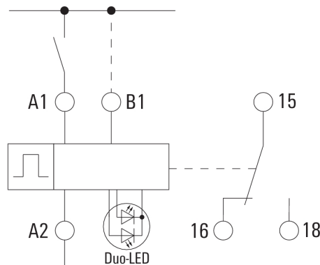
Wiring example
