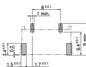
(2 circuits 8 mm pitch)
