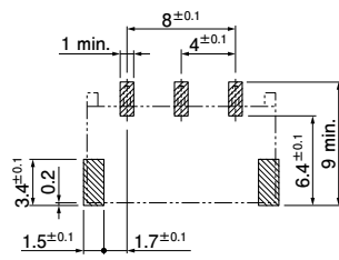
(4 circuits 4 mm pitch with post removed)
