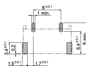
(2 circuits 8 mm pitch plugged up)
