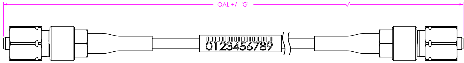
FIG 1 WF-15-S-75TP-75TP-XXXX SHOWN (PROTECTIVE CAPS NOT SHOWN FOR CLARITY)
