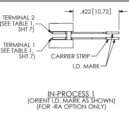
FIG 5 -RA OPTION DIFFERENT AS SHOWN, OTHERWISE SAME AS FIG 1
