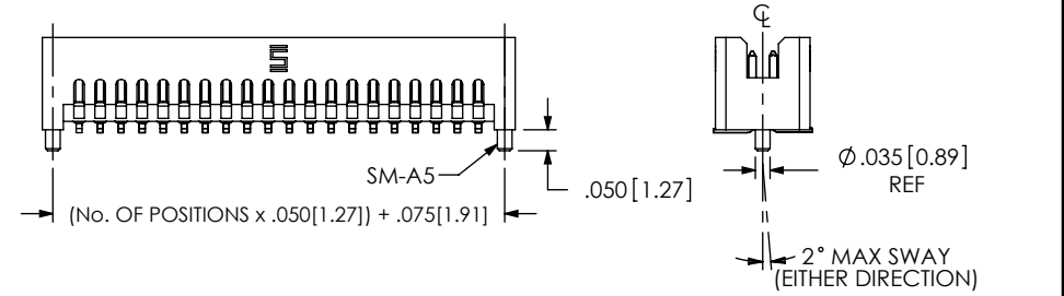
FIG 9 -SA OPTION: STAKED ALIGNMENT PIN DIFFERENT AS SHOWN, OTHERWISE SAME AS FIG 1
