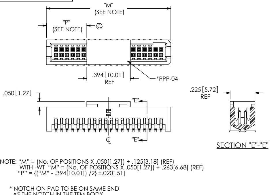
FIG 7 -P OPTION DIFFERENT AS SHOWN, OTHERWISE SAME AS FIG 1 (PAD TO BE POSITIONED ON C.L. AS SHOWN)
