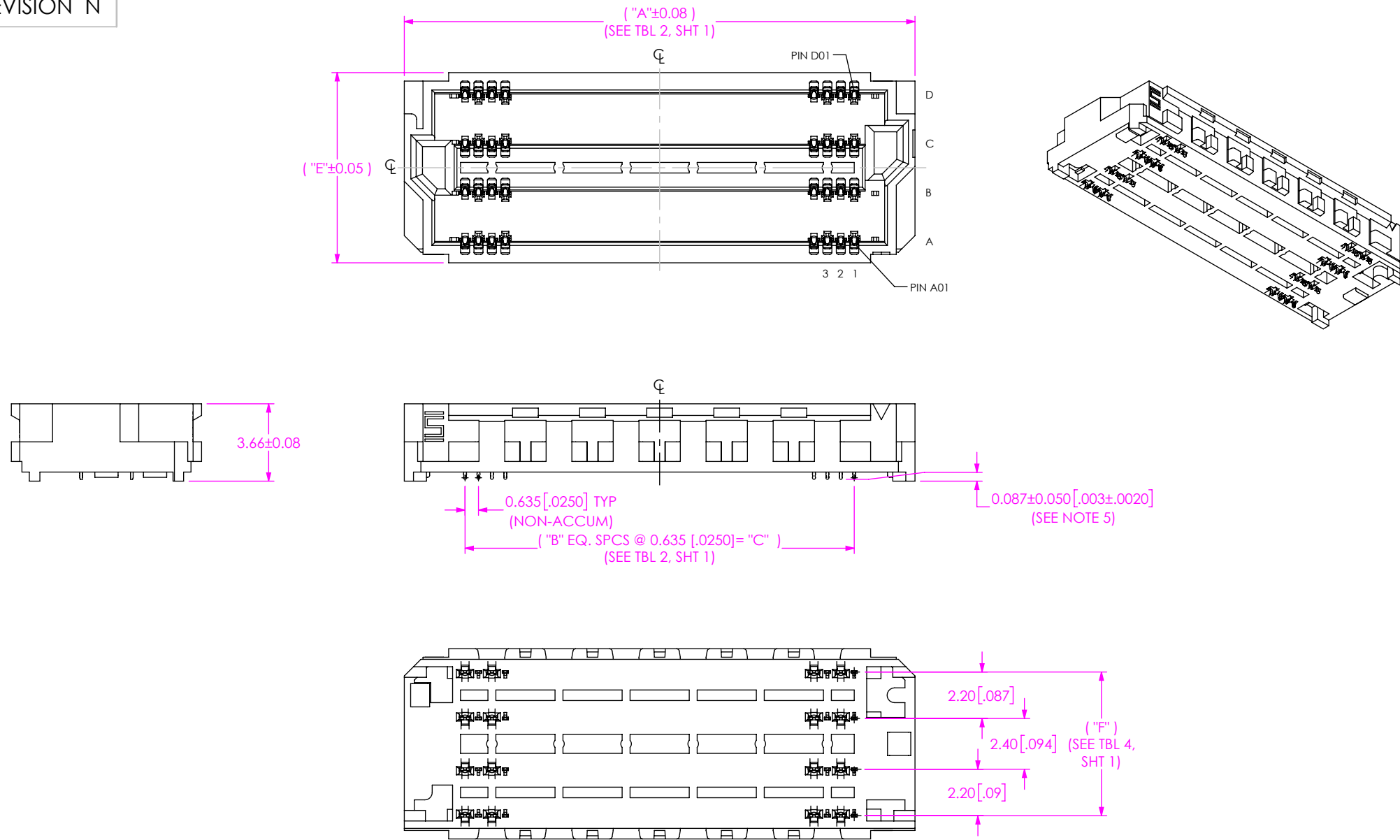
FIG 8 APF6-030-03.5-XXX-04-0 SHOWN (NO SOLDER BALL OPTION) (SOME CENTER FEATURES REMOVED FOR CLARITY)
