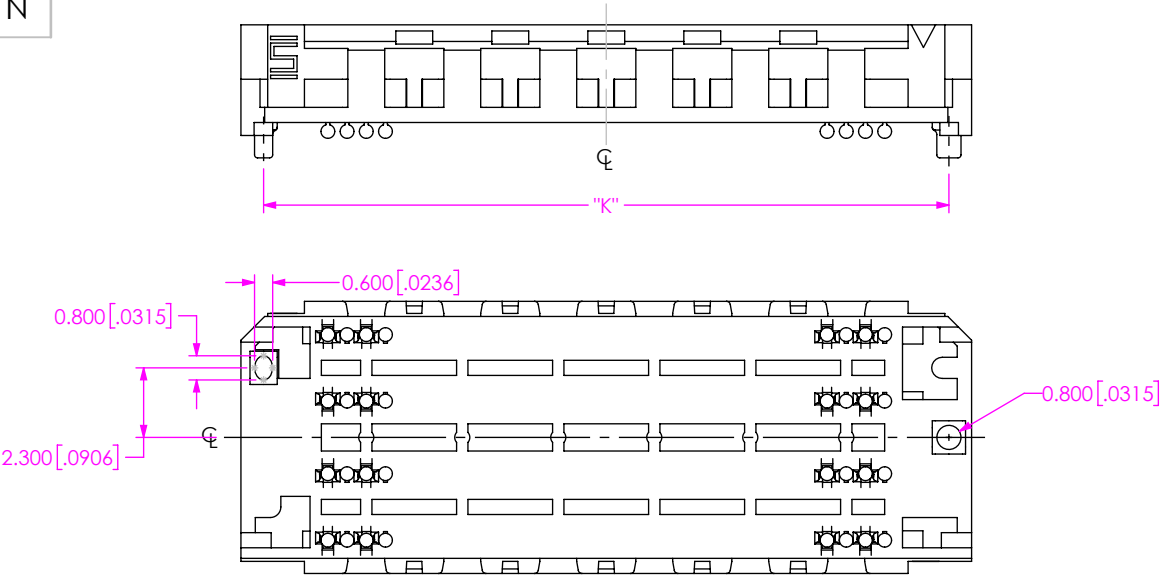
FIG 3 -A: ALIGNMENT PIN APF6-030-03.5-XXX-04-X-A SHOWN (SAME AS FIG 1, EXCEPT AS SHOWN) (SOME CENTER FEATURES REMOVED FOR CLARITY)
