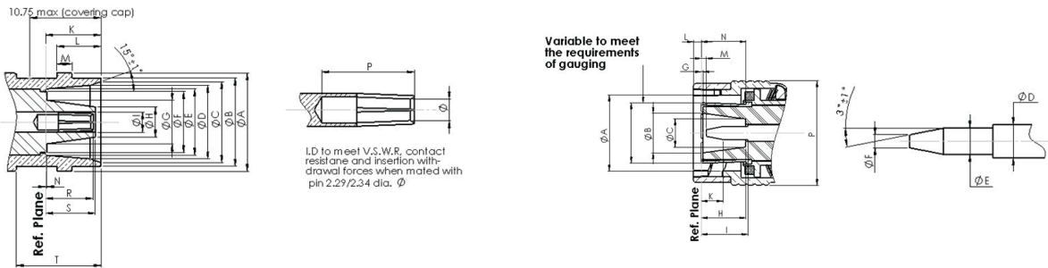
CEI DIMENSIONS (IN MM)
