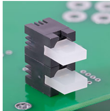
LED Mount, Self Retaining, Vertical, 16mm, 2,3 Lead, Rectangular, Extruded PVC, Black
