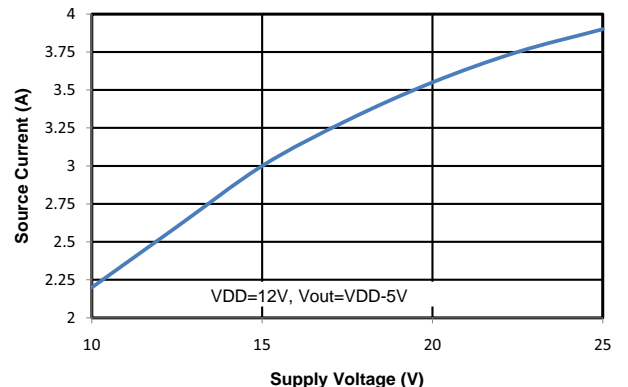
Figure 17. Output Source Current vs. Supply Voltage
