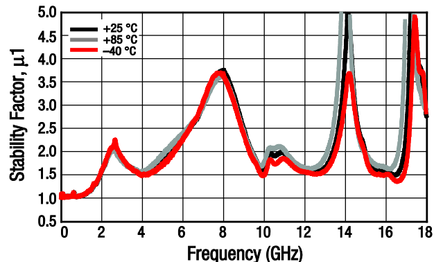
Figure 25. Stability Factor ( \mu_1 ) vs Frequency and Temperature, Wide Band
