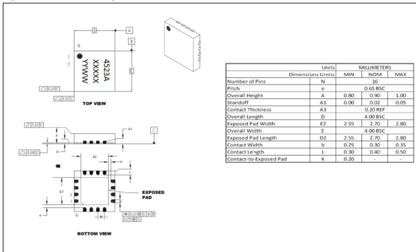
Figure 5.1 PQFN-16 Package Dimensions
