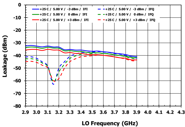
LO to IF Leakage vs. LO Power [Low Side LO]
