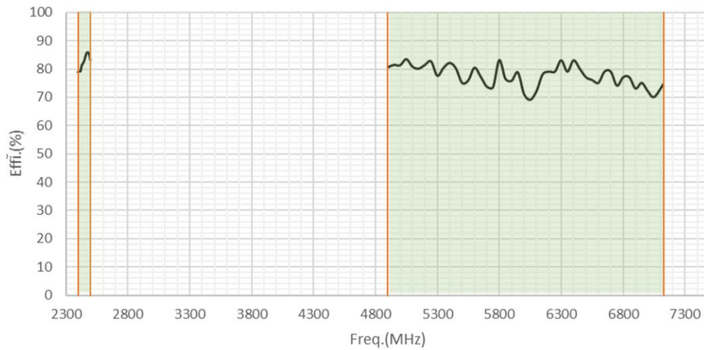
Efficiency vs Frequency Measured in PSU 20230718
