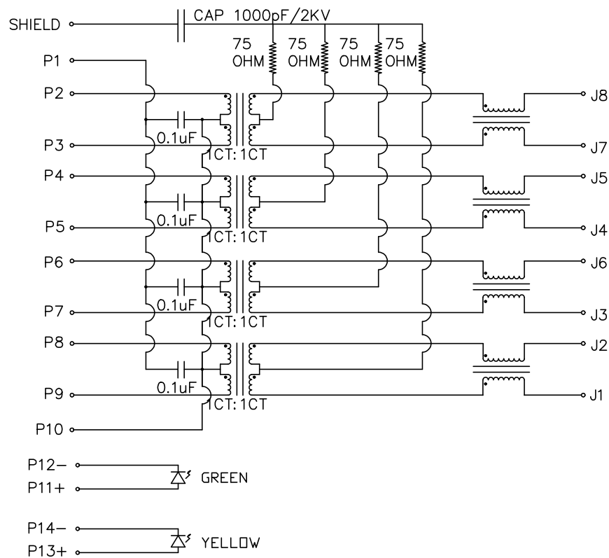
SCHEMATIC
