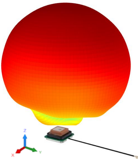
L1 3D RHCP Pattern @1575 MHz
