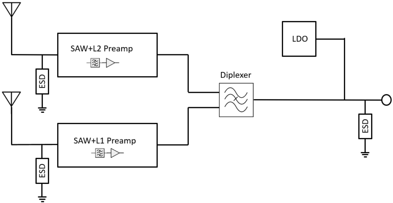
Active Antenna Block Diagram
