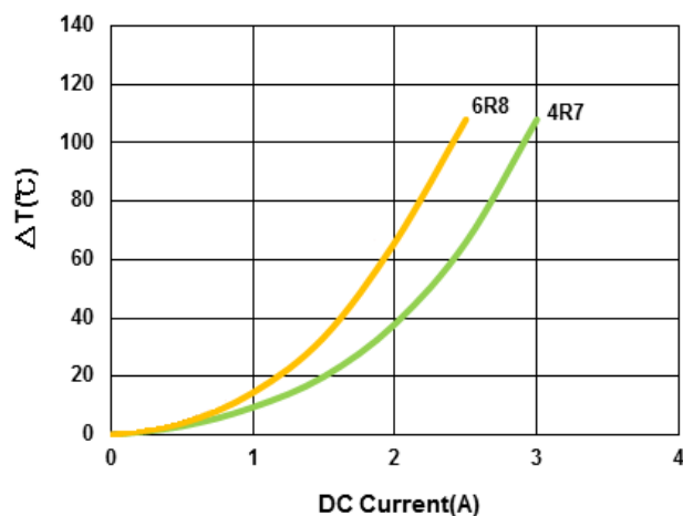
Temperature Change v.s DC Current
