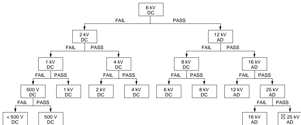
Fig. 7 Passive component HBM ESD test flow diagram (DC = Direct Contact Discharge, AD = Air Discharge)
