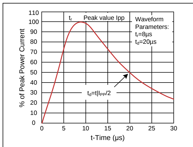
Figure 2. Pulse Waveforms
