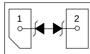
Pin Configuration
