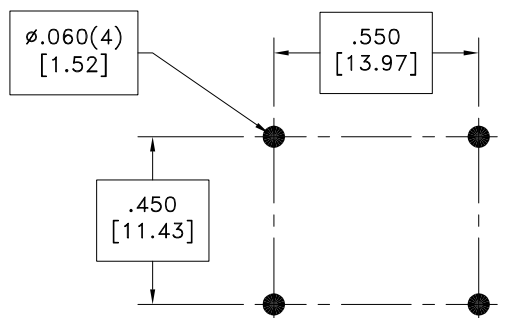
RECOMMENDED P.C. PATTERN, COMPONENT SIDE
