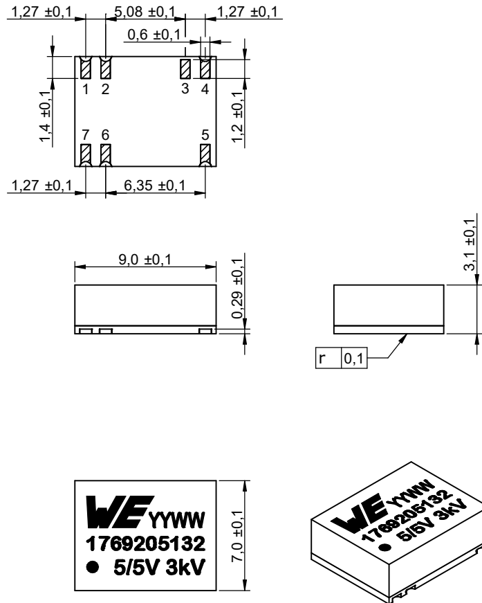
Figure 19: Physical dimensions.
