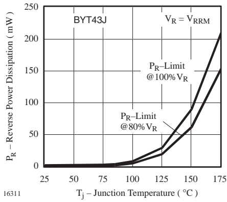
Figure 7. Max. Reverse Power Dissipation vs. Junction Temperature
