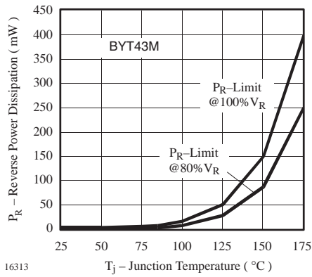
Figure 8. Max. Reverse Power Dissipation vs. Junction Temperature
