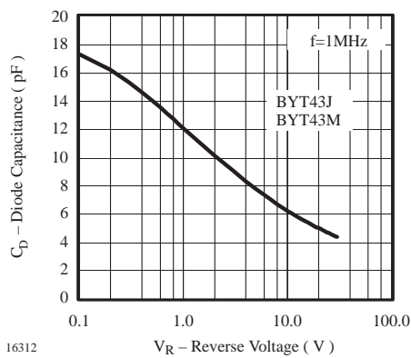
Figure 9. Diode Capacitance vs. Reverse Voltage
