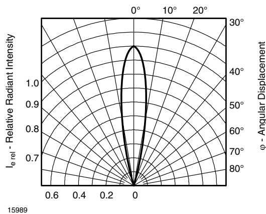
Fig. 7 - Relative Radiant Intensity vs. Angular Displacement
