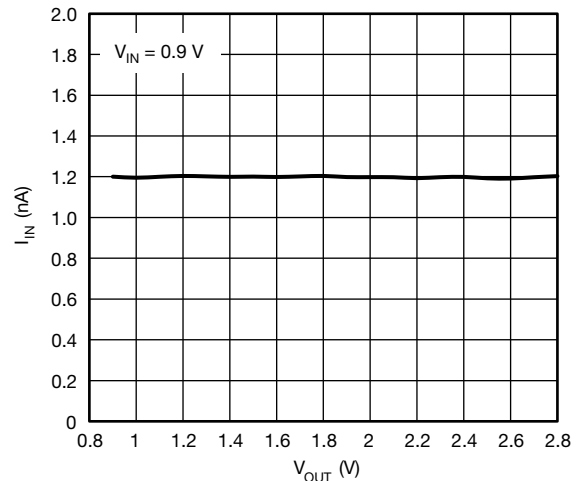
Fig. 14 - Reverse Blocking Current vs. Output Voltage
