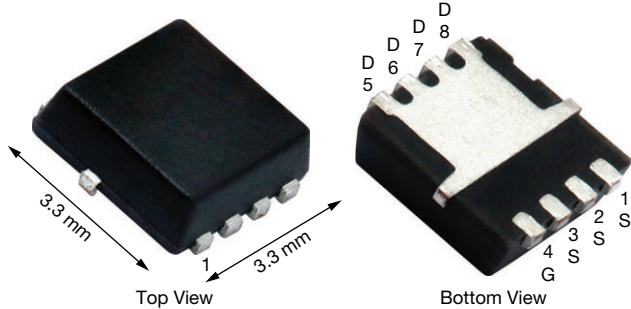
PowerPAK® 1212-8 Single
