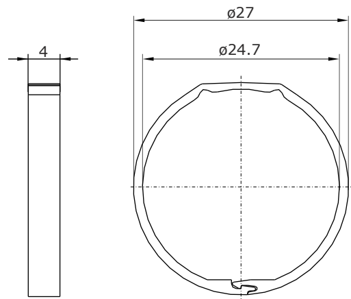
Main Dimensions colored ring
