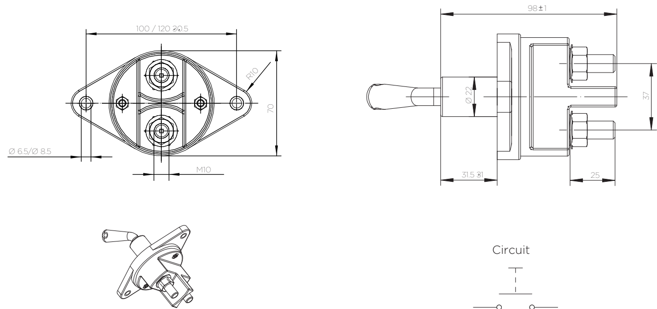
1-pole with longflange
