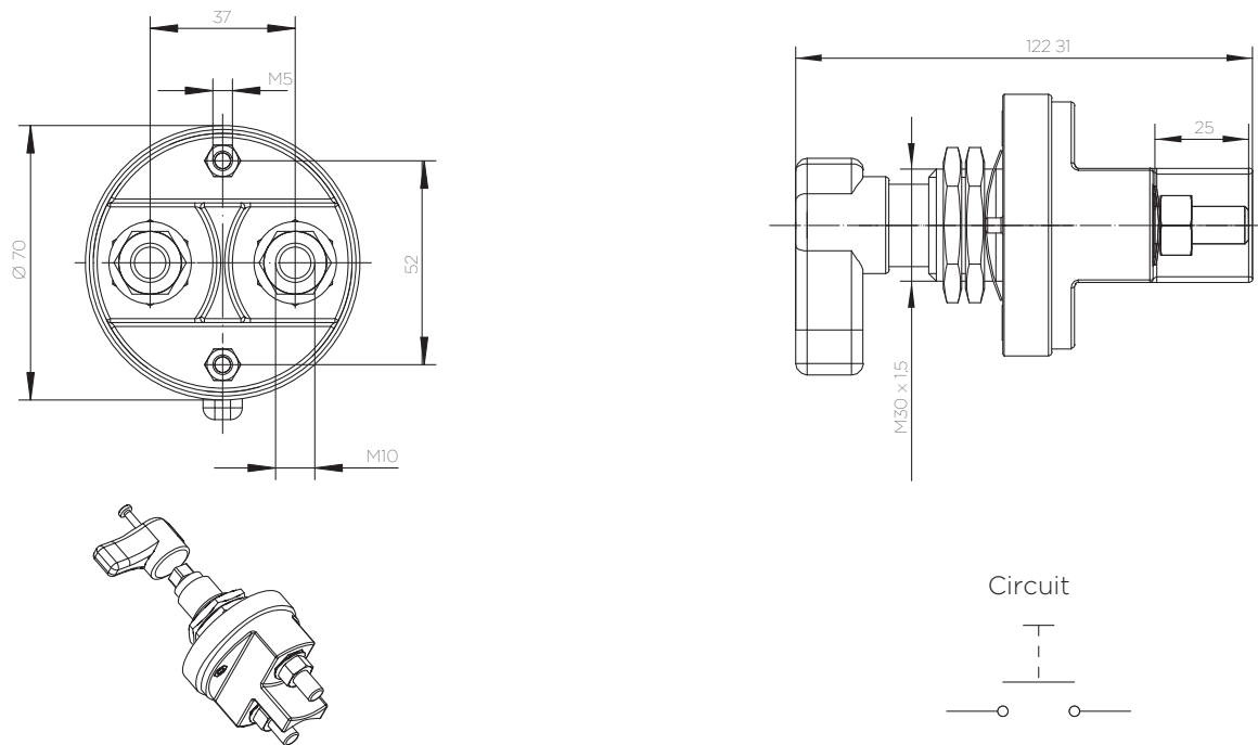
1-pole with central mounting
