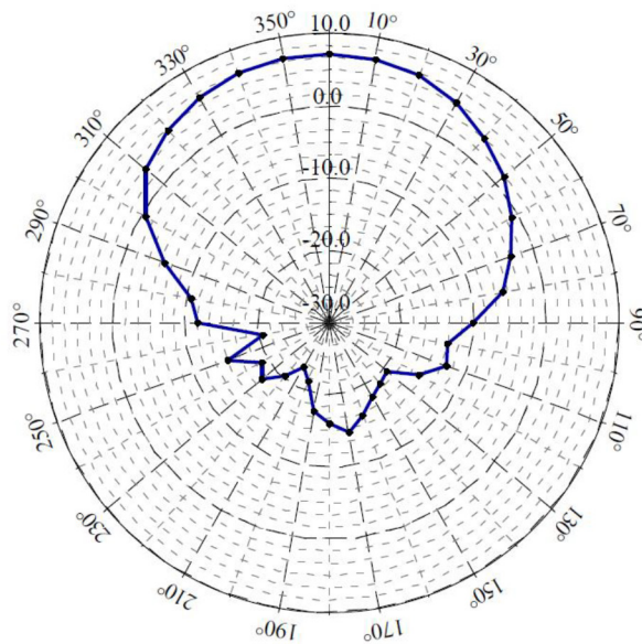
Vertical-to-Vertical Polarization Azimuth (X, Y, or E-plane)
