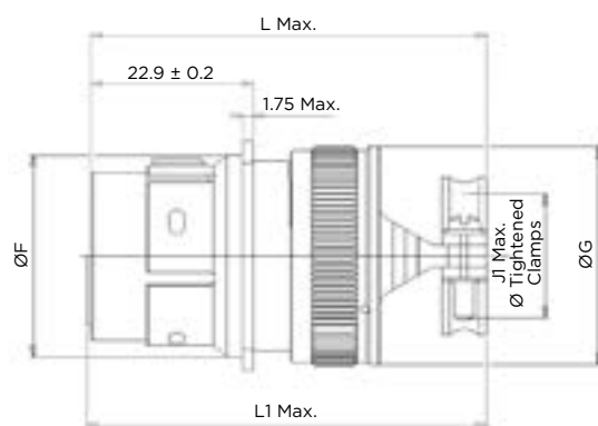
DBAS 970 With Straight Cable Clamp (059)
