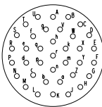
25-37 37 Size 16 Contacts
