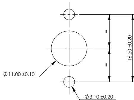
PANEL CUT-OUT DETAIL
