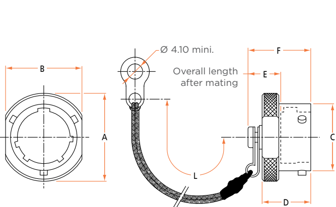
ATTACHED TO ACCESSORY (CABLE CLAMP) TYPE 06 C
